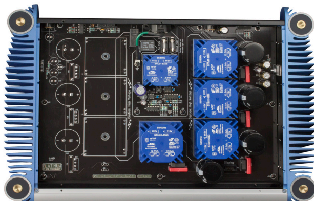
Signature Transport Power Base with 8 transformers.
